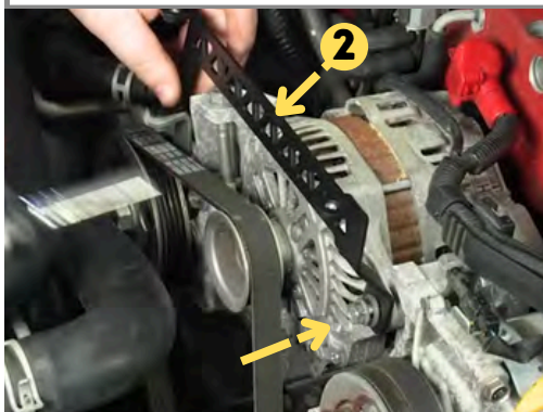
Step 5: Install the IAG Cover Bracket with the factory 12mm bolt. Do not tighten.
