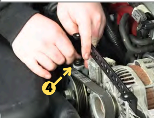
Step 6: Install provided 10mm bolt onto the Cover Bracket. Do not tighten.
