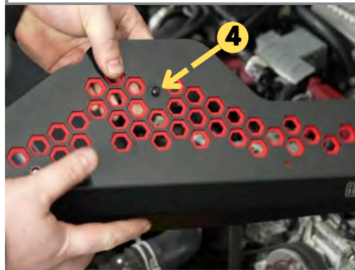
Step 9: Use provided 2.5mm Allen bolt, assemble the Color Plate to the Alternator Cover. Do not tighten.
