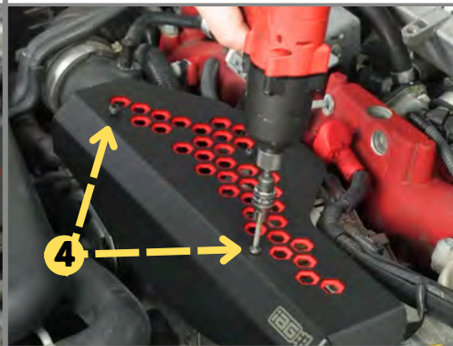
Step 9: Use provided 4mm Allen bolts, install Alternator Cover. Ensure color plate is centered, then tighten hardware.
